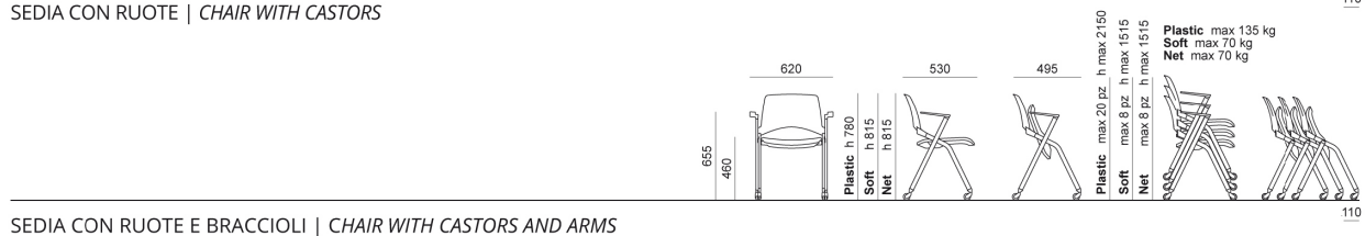
SEDIA CON RUOTE E BRACCIOLI | CHAIR WITH CASTORS AND ARMS
